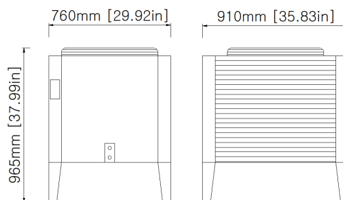
EXTERNAL RADIATOR
